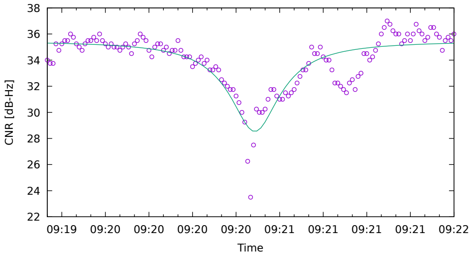
CNR fit for G08 on XiaomiMi8 - drive 3 (DOY262)
