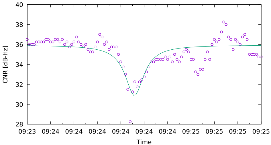
CNR fit for G08 on XiaomiMi8 - drive 5 (DOY262)
