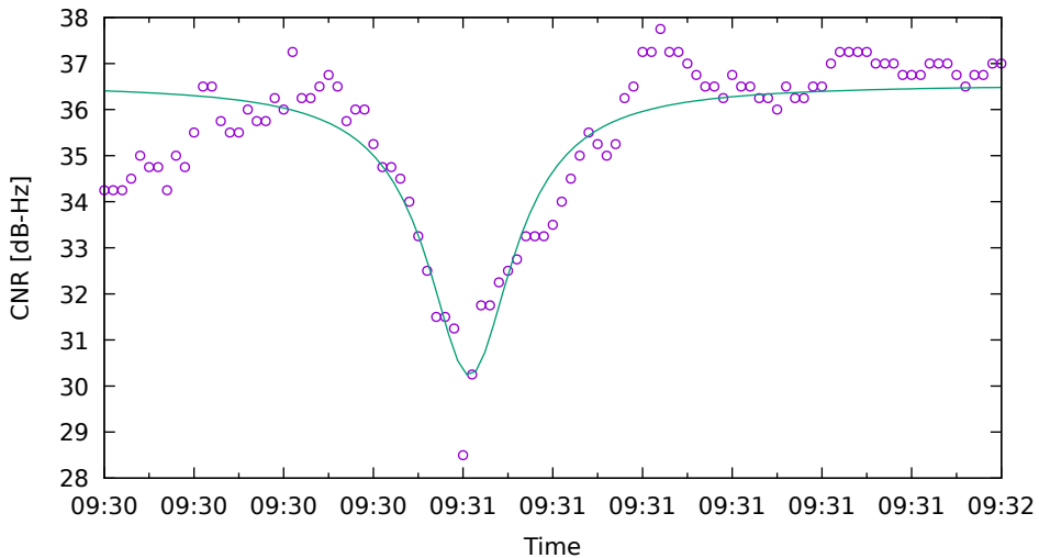
CNR fit for G08 on XiaomiMi8 - drive 8 (DOY262)
