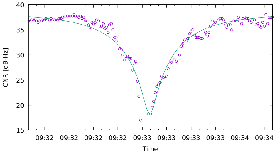
CNR fit for G08 on XiaomiMi8 - drive 9 (DOY262)
