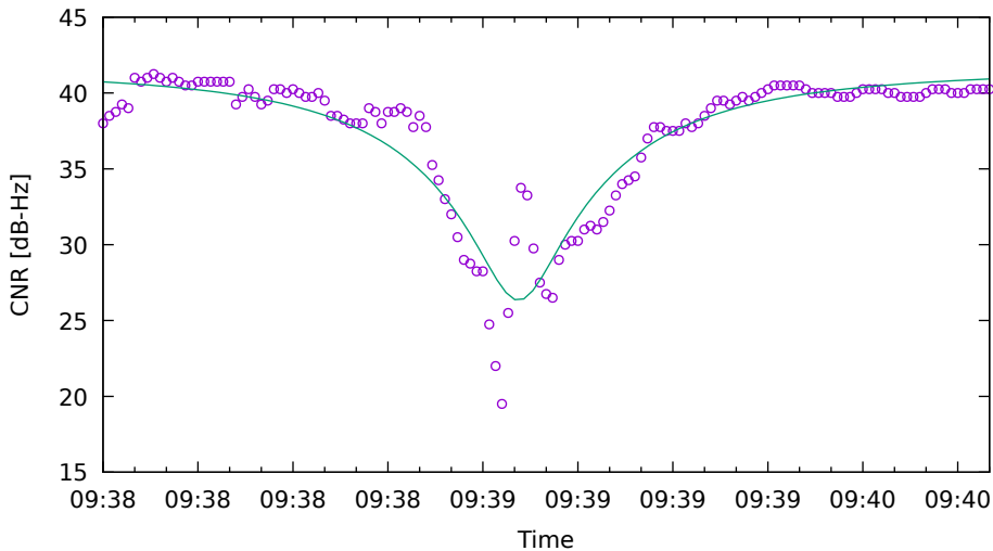
CNR fit for G17 on XiaomiMi8 - drive 12 (DOY262)
