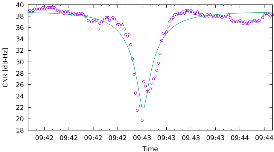
CNR fit for G17 on XiaomiMi8 - drive 14 (DOY262)
