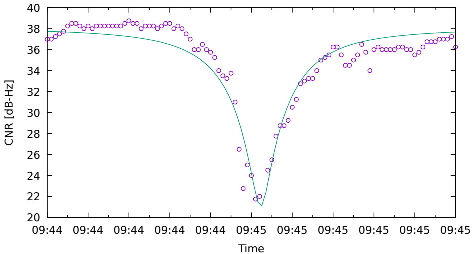
CNR fit for G17 on XiaomiMi8 - drive 15 (DOY262)
