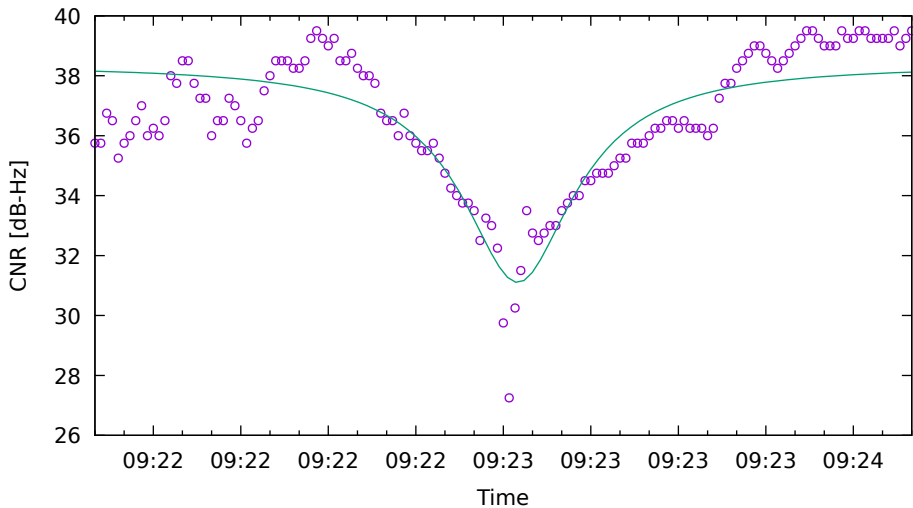
CNR fit for G17 on XiaomiMi8 - drive 4 (DOY262)
