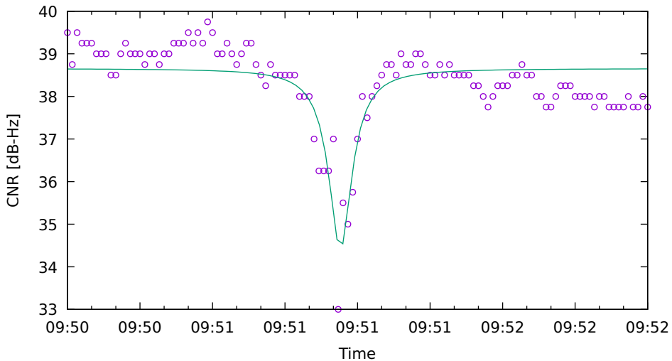
CNR fit for G19 on XiaomiMi8 - drive 18 (DOY262)
