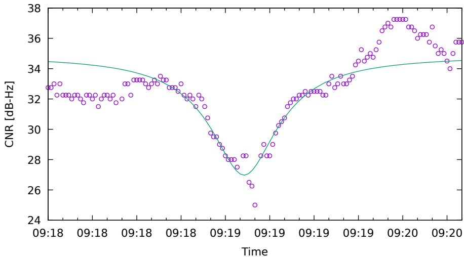
CNR fit for G19 on XiaomiMi8 - drive 2 (DOY262)
