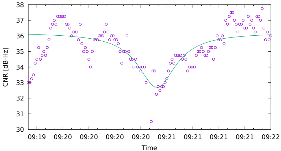
CNR fit for G19 on XiaomiMi8 - drive 3 (DOY262)
