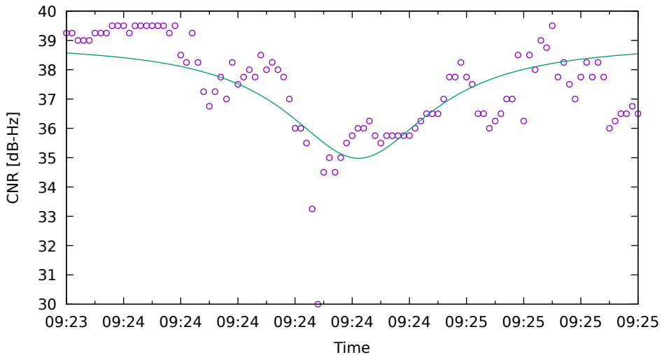
CNR fit for G19 on XiaomiMi8 - drive 5 (DOY262)
