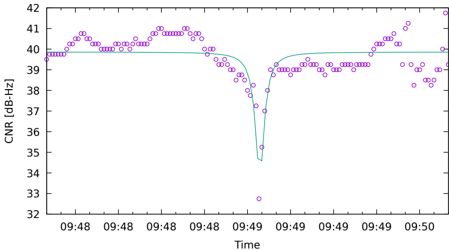
CNR fit for G21 on XiaomiMi8 - drive 17 (DOY262)
