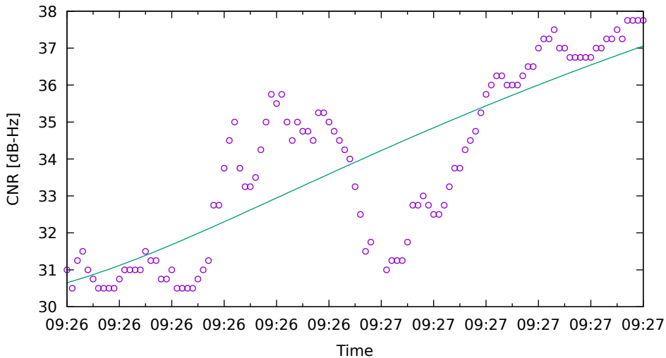
CNR fit for G21 on XiaomiMi8 - drive 6 (DOY262)
