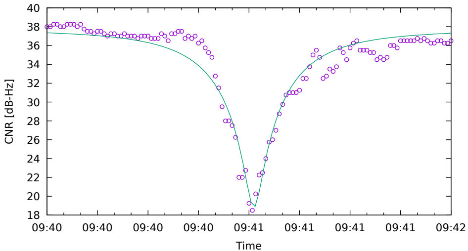
CNR fit for G22 on XiaomiMi8 - drive 13 (DOY262)
