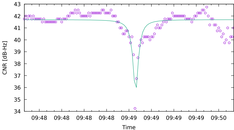
CNR fit for G22 on XiaomiMi8 - drive 17 (DOY262)
