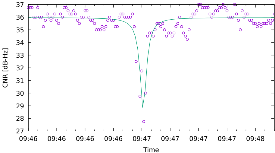
CNR fit for R07 on XiaomiMi8 - drive 16 (DOY262)
