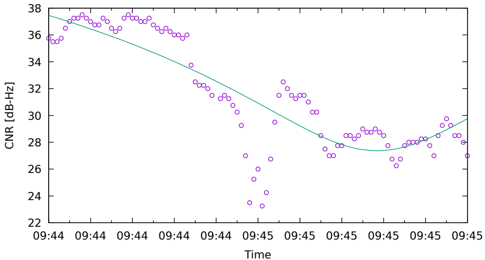
CNR fit for R24 on XiaomiMi8 - drive 15 (DOY262)
