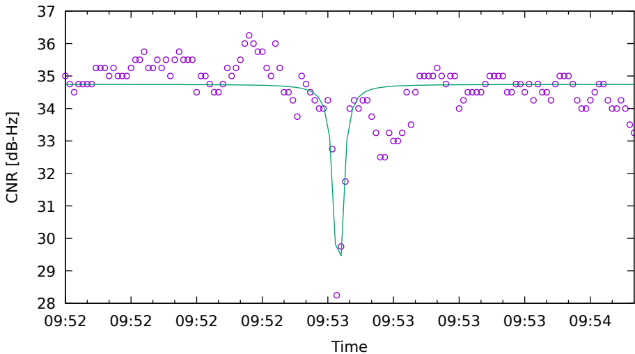
CNR fit for R24 on XiaomiMi8 - drive 19 (DOY262)
