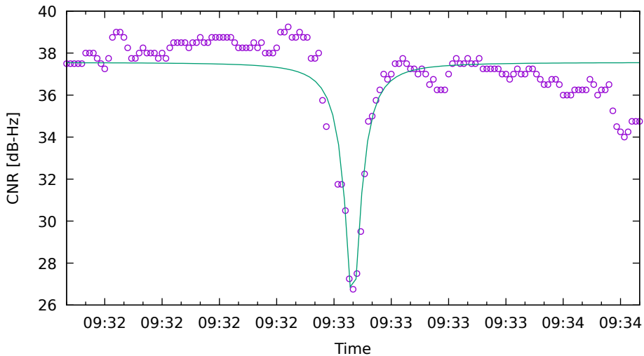
CNR fit for R24 on XiaomiMi8 - drive 9 (DOY262)
