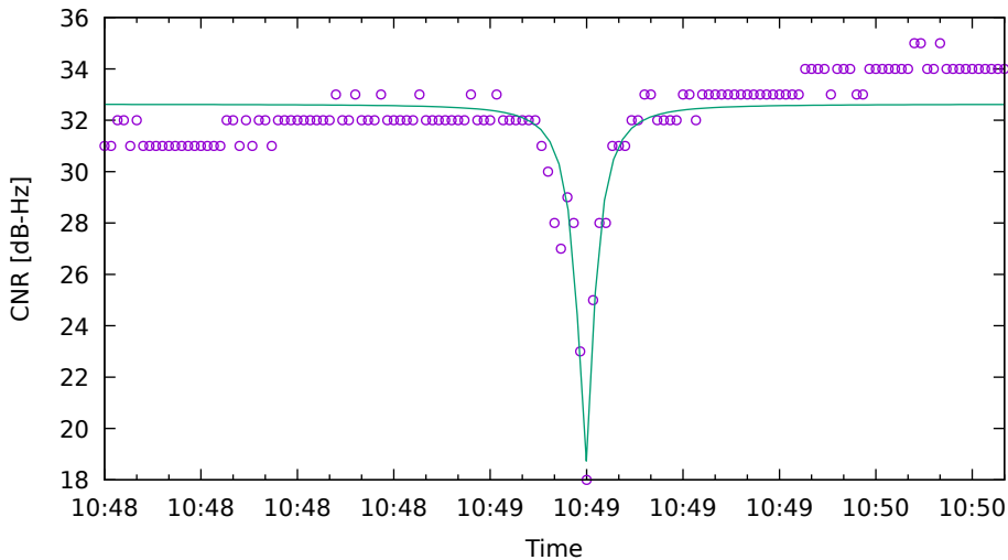
CNR fit for C06 on HuaweiP40 - drive 4 (DOY262)
