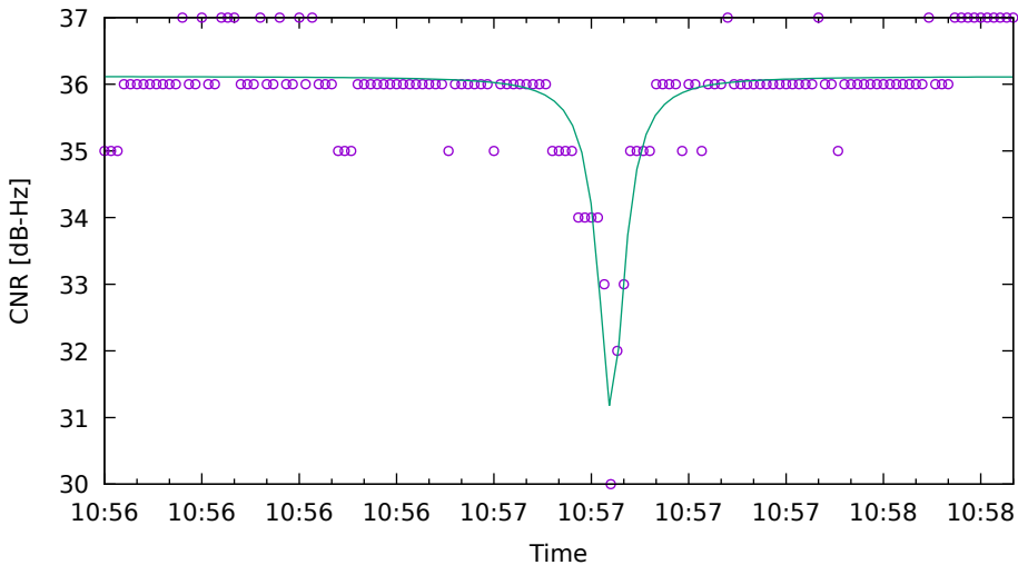
CNR fit for C06 on HuaweiP40 - drive 8 (DOY262)
