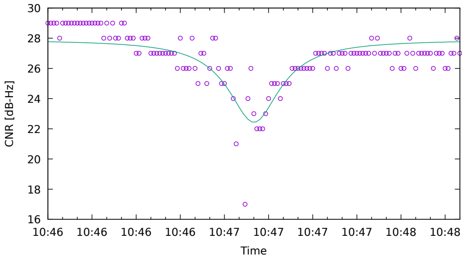
CNR fit for C09 on HuaweiP40 - drive 3 (DOY262)
