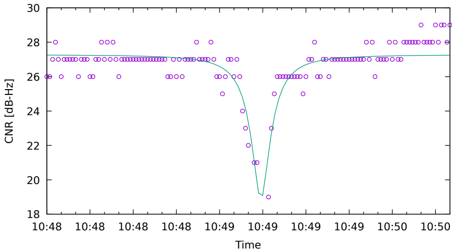
CNR fit for C09 on HuaweiP40 - drive 4 (DOY262)
