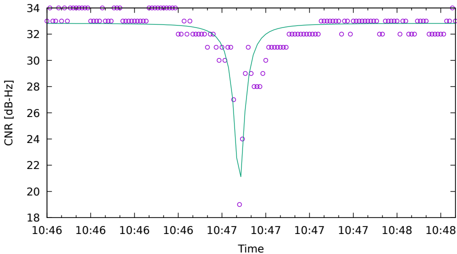
CNR fit for C16 on HuaweiP40 - drive 3 (DOY262)
