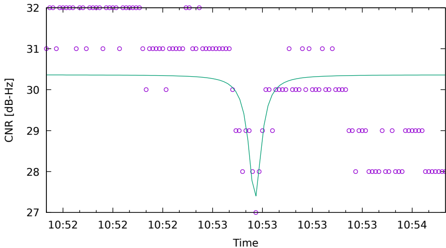
CNR fit for C16 on HuaweiP40 - drive 6 (DOY262)
