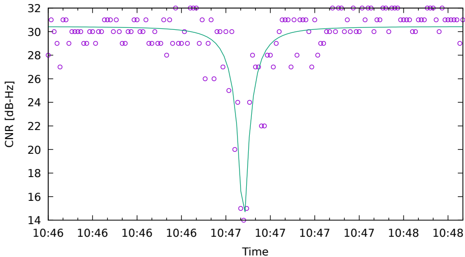
CNR fit for C26 on HuaweiP40 - drive 3 (DOY262)
