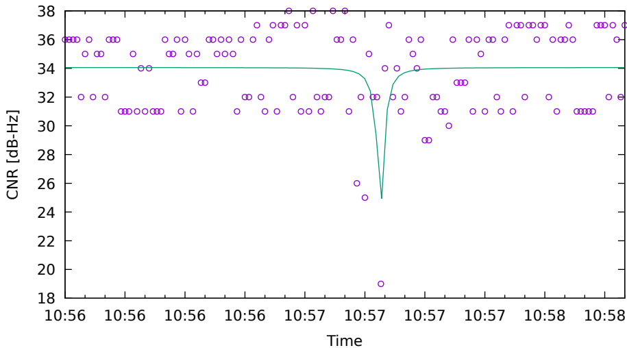
CNR fit for C26 on HuaweiP40 - drive 8 (DOY262)
