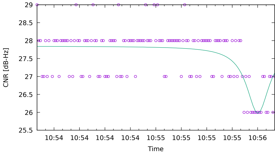
CNR fit for E05 on HuaweiP40 - drive 7 (DOY262)
