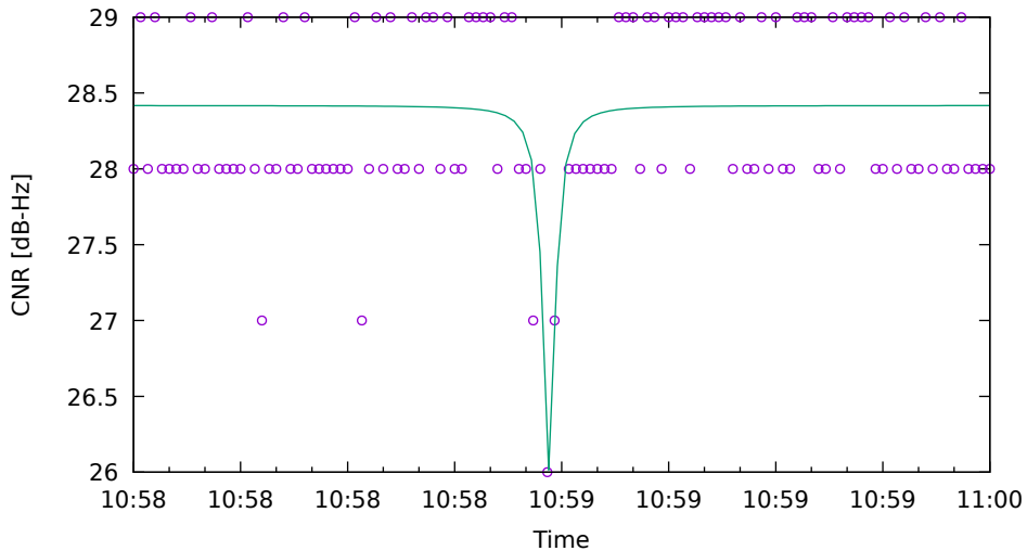
CNR fit for E05 on HuaweiP40 - drive 9 (DOY262)
