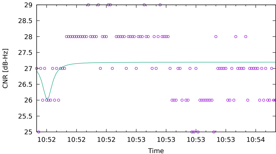
CNR fit for E36 on HuaweiP40 - drive 6 (DOY262)
