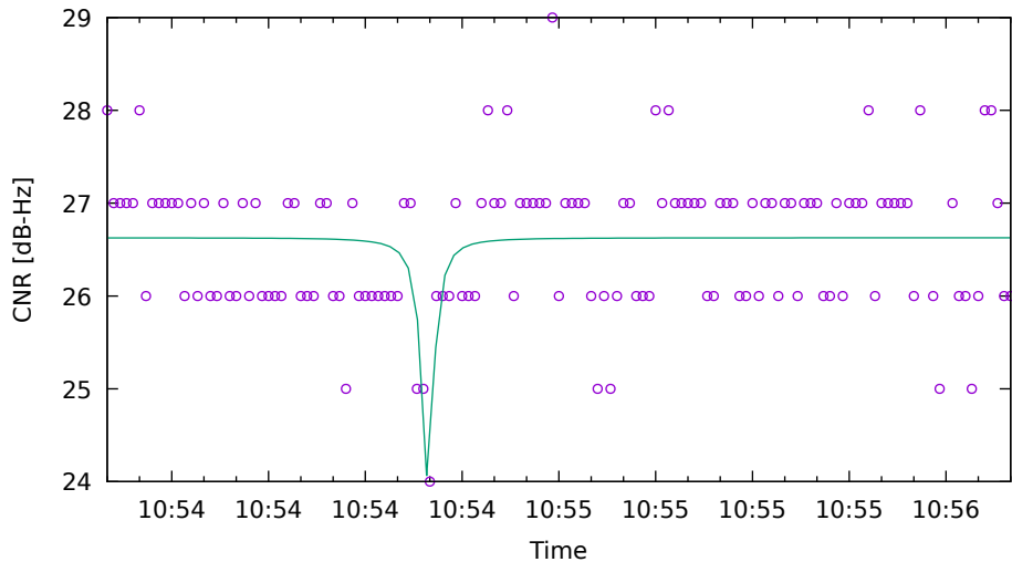
CNR fit for E36 on HuaweiP40 - drive 7 (DOY262)
