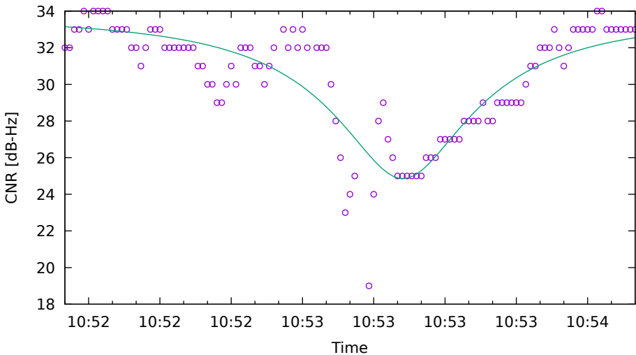
CNR fit for G03 on HuaweiP40 - drive 6 (DOY262)
