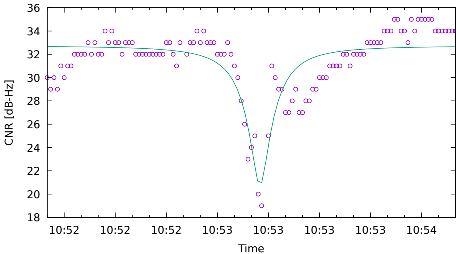
CNR fit for G04 on HuaweiP40 - drive 6 (DOY262)
