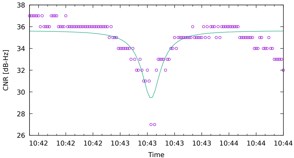
CNR fit for G09 on HuaweiP40 - drive 1 (DOY262)
