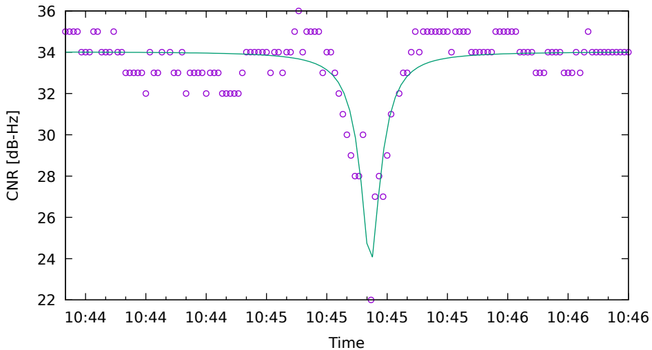
CNR fit for G09 on HuaweiP40 - drive 2 (DOY262)
