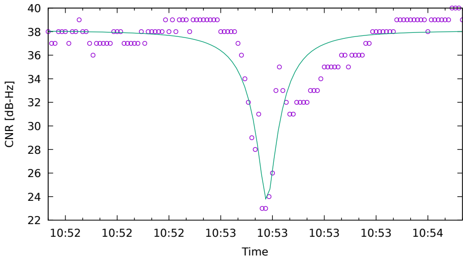
CNR fit for G09 on HuaweiP40 - drive 6 (DOY262)
