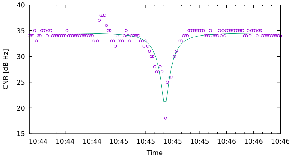
CNR fit for G19 on HuaweiP40 - drive 2 (DOY262)
