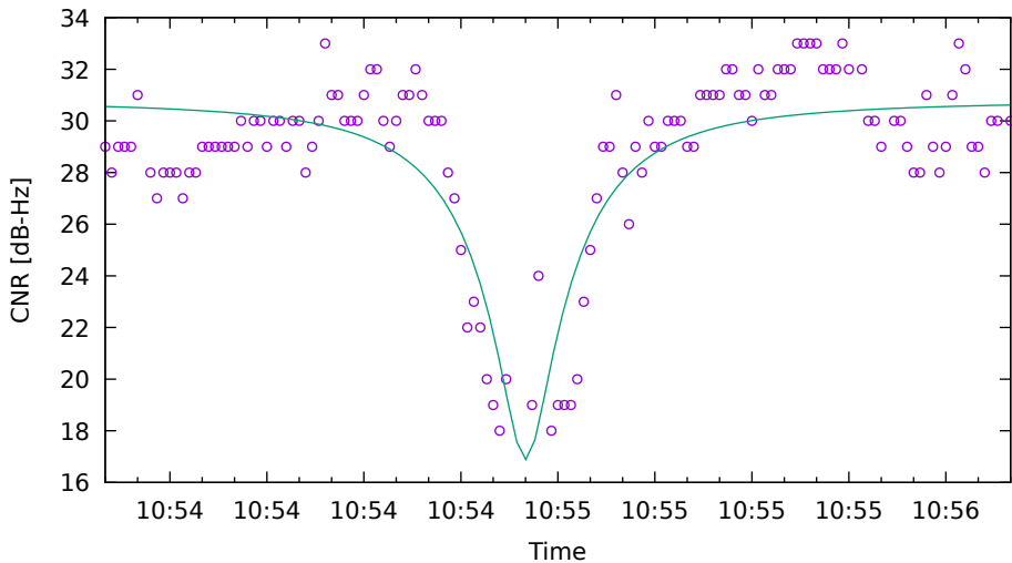
CNR fit for G19 on HuaweiP40 - drive 7 (DOY262)
