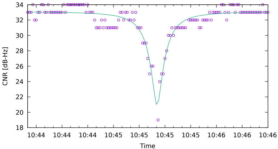
CNR fit for G21 on HuaweiP40 - drive 2 (DOY262)
