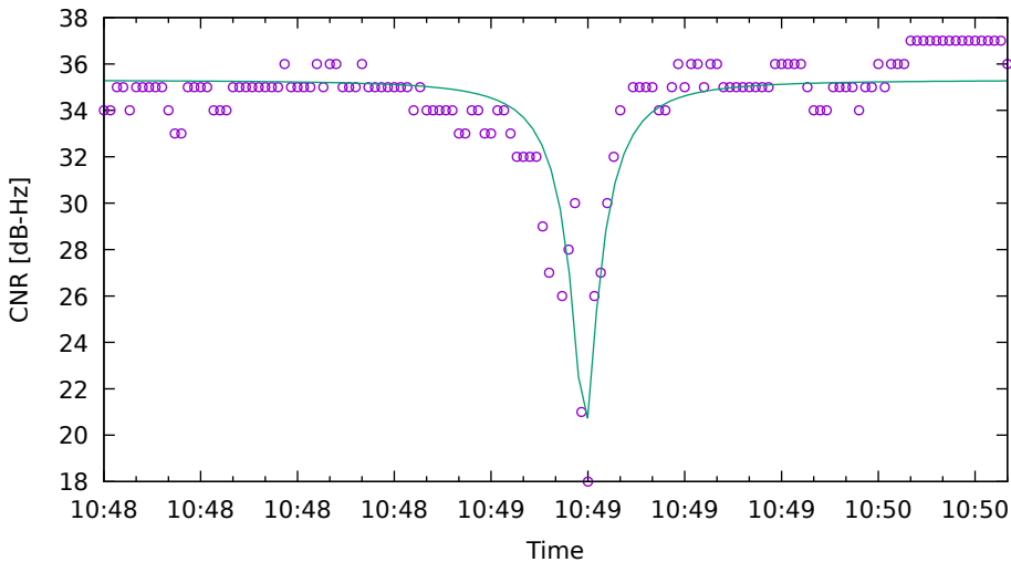
CNR fit for G31 on HuaweiP40 - drive 4 (DOY262)
