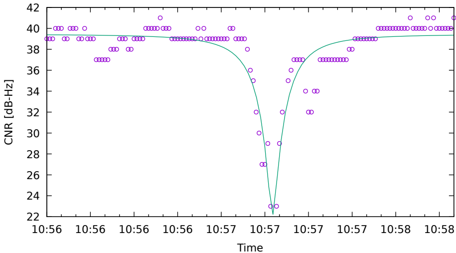
CNR fit for G31 on HuaweiP40 - drive 8 (DOY262)
