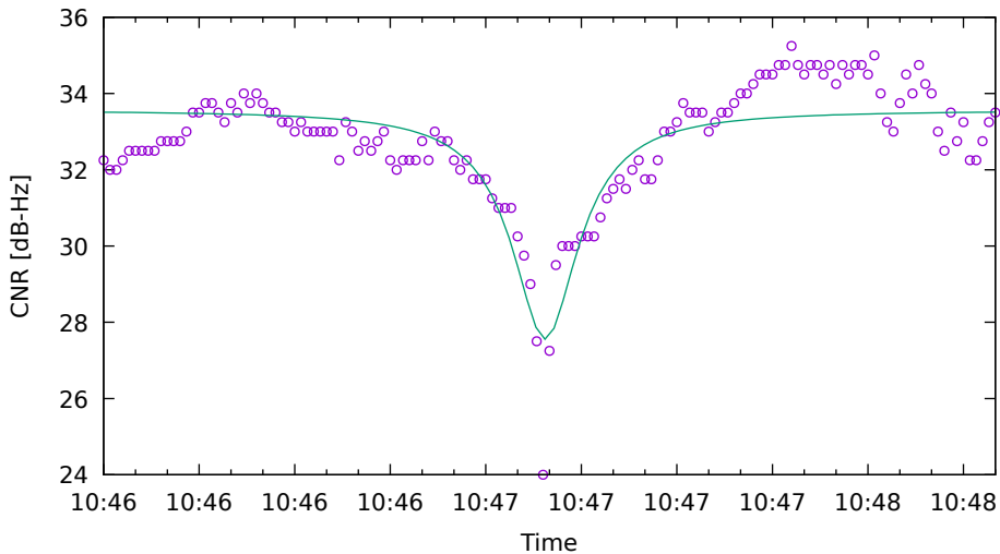
CNR fit for E05 on XiaomiMi8 - drive 3 (DOY262)
