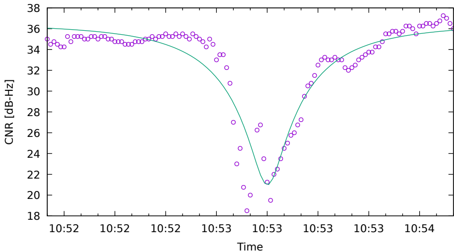
CNR fit for E05 on XiaomiMi8 - drive 6 (DOY262)
