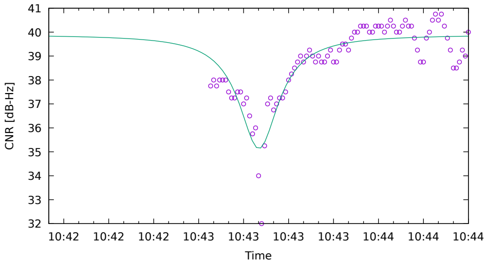
CNR fit for E09 on XiaomiMi8 - drive 1 (DOY262)
