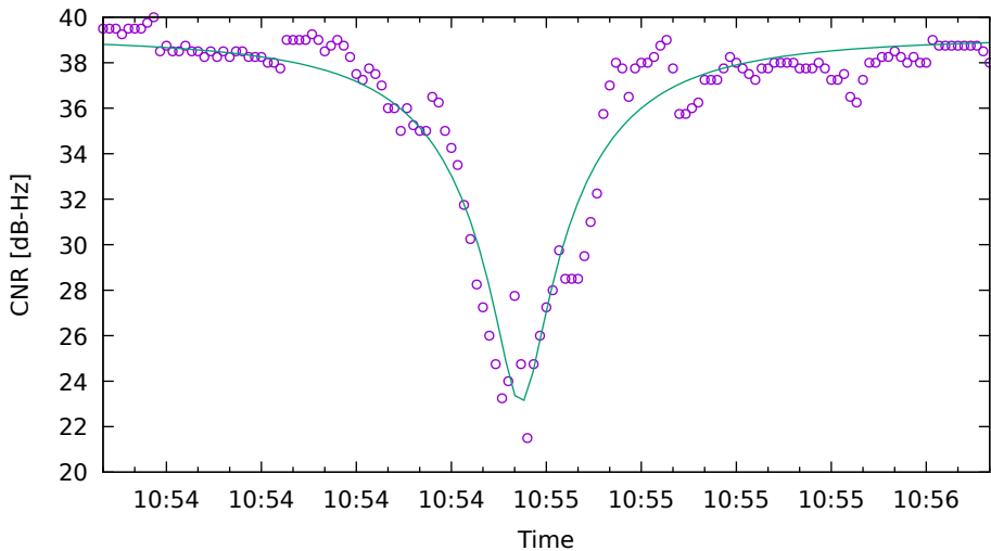
CNR fit for E09 on XiaomiMi8 - drive 7 (DOY262)
