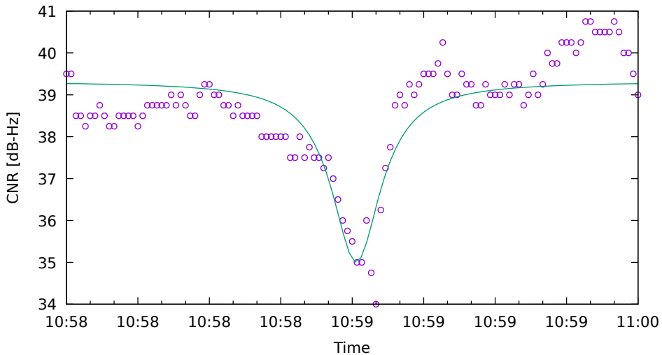
CNR fit for E09 on XiaomiMi8 - drive 9 (DOY262)
