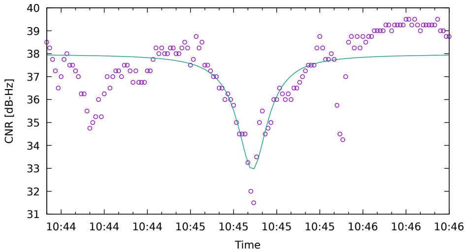
CNR fit for E34 on XiaomiMi8 - drive 2 (DOY262)
