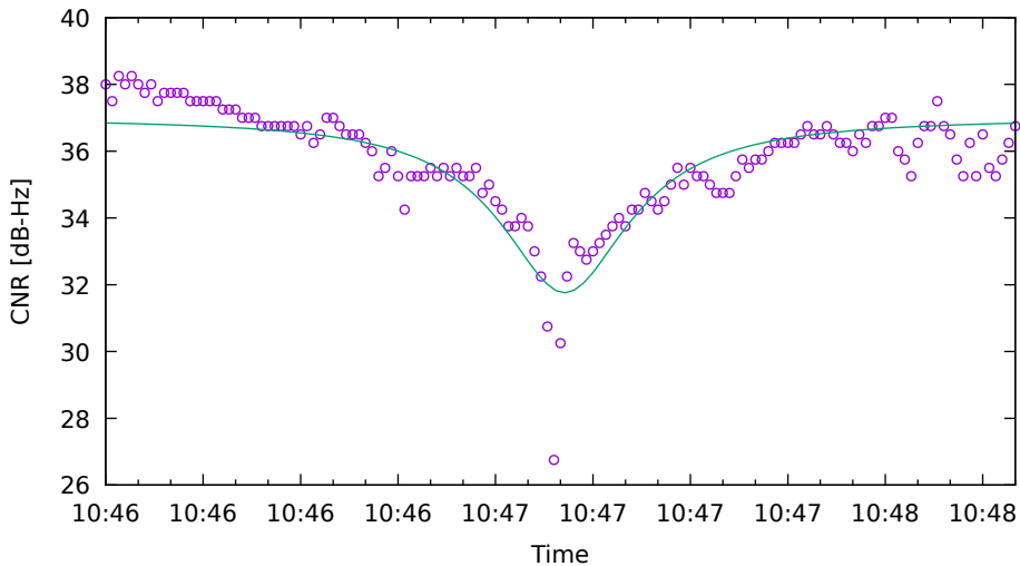
CNR fit for E36 on XiaomiMi8 - drive 3 (DOY262)
