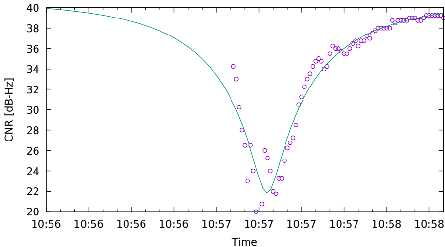
CNR fit for E36 on XiaomiMi8 - drive 8 (DOY262)
